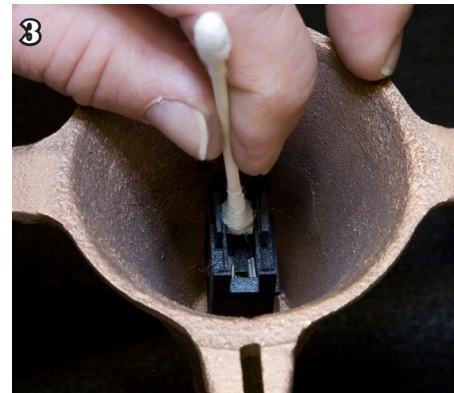
3 Clean all four socket contacts using cotton swab (with grease). Use up-and-down and twisting motion to scrub contacts. Do not allow grease to contact plastic between contact pairs.*
